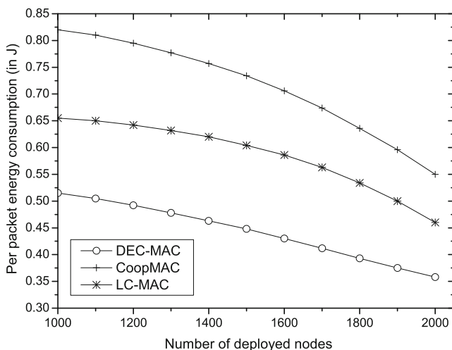
Fig. 8 Per-packet energy consumption vs. number of deployed nodes
