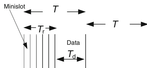
Fig. 2 Time slots for two data bursts
