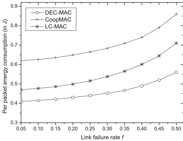
Fig. 13 Energy efficiency vs. link failure rate
