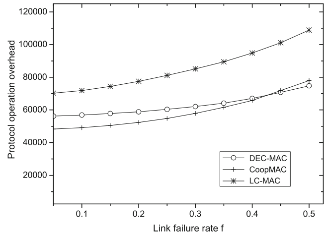
Fig. 15 Protocol operation overhead vs. link failure rate
