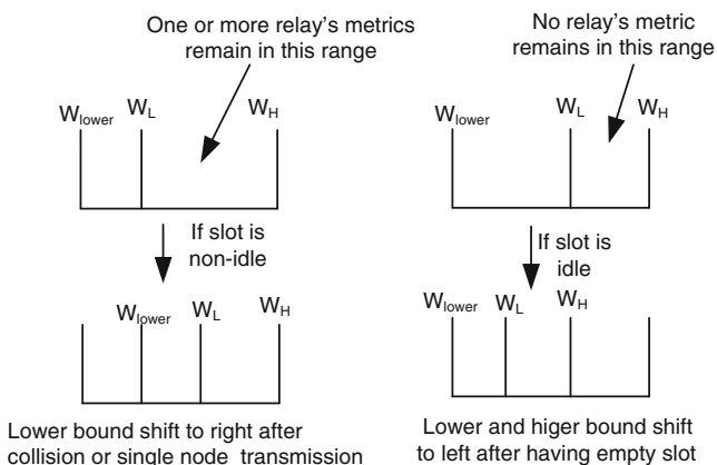
Fig. 3 Upper and lower threshold update procedure
