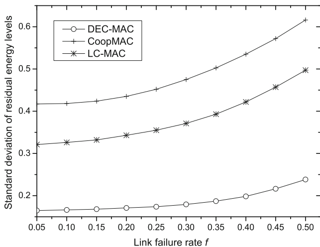
Fig. 14 Standard deviation of residual energy vs. link failure rate
