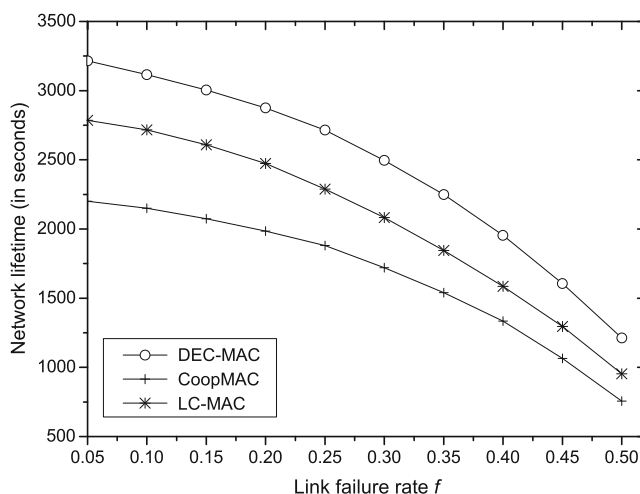
Fig. 12 Network lifetime vs. link failure rate
