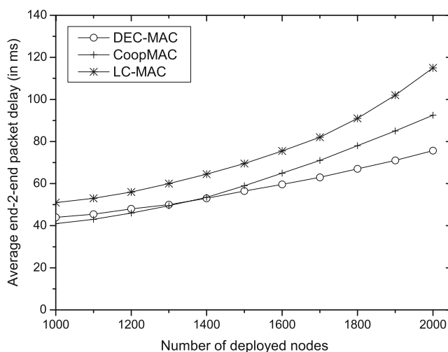
Fig. 6 Average end-to-end delay vs. number of deployed nodes
