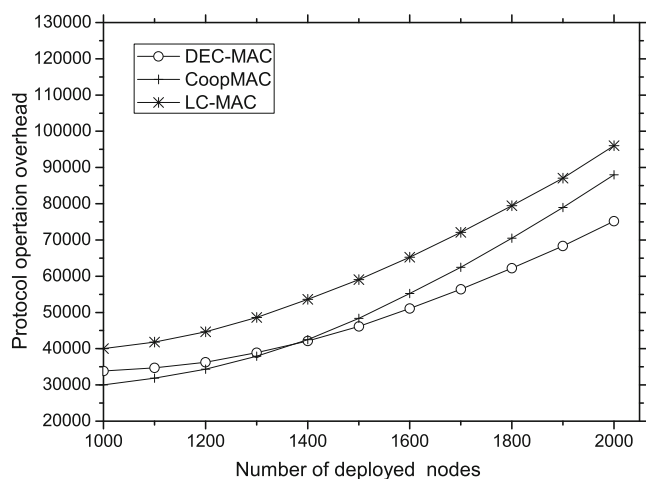
Fig. 10 Protocol operation overhead vs. number of deployed of nodes
