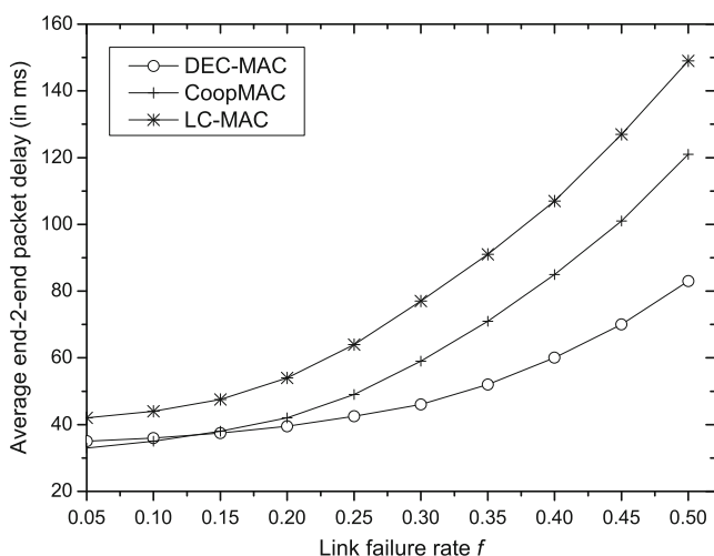
Fig. 11 Average end-to-end delay vs. link failure rate
