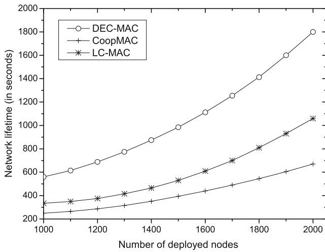
Fig. 7 Network lifetime vs. number of deployed nodes
